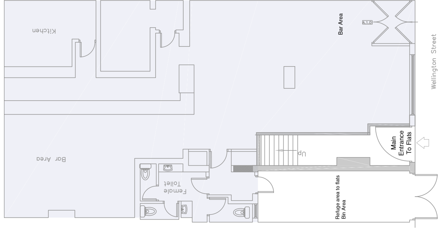
23 Wellington Street, Leicester Ground Floor Layout
