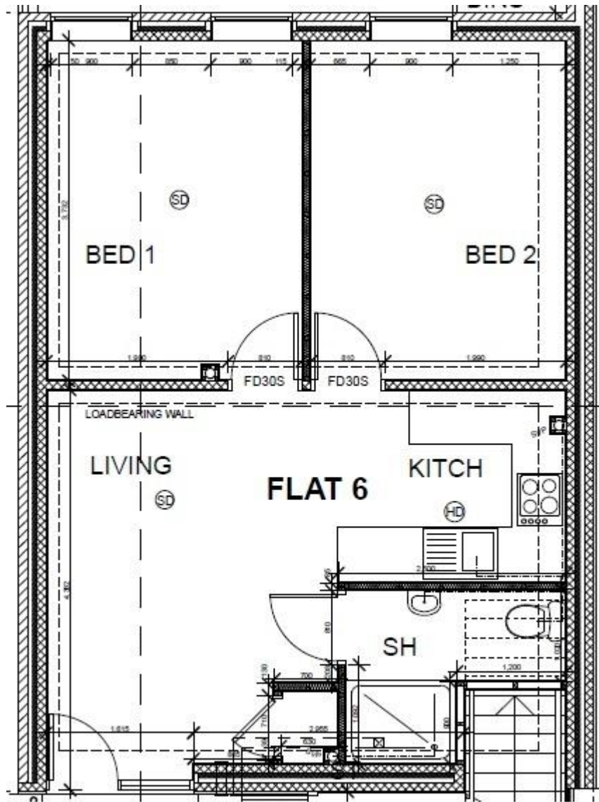
Ground Floor
